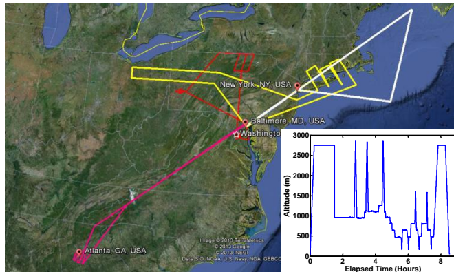
Figure 11. Example flight patterns for WINTER.
