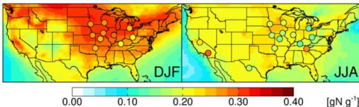
Figure 6. The fraction of inorganic nitrogen in mean surface fine particulate matter mass during winter (left) and summer (right). Measurements from the Midwest Ammonia Monitoring Project (dots) are overlaid on Geos-Chem output. Taken from Heald et al. [2012].
