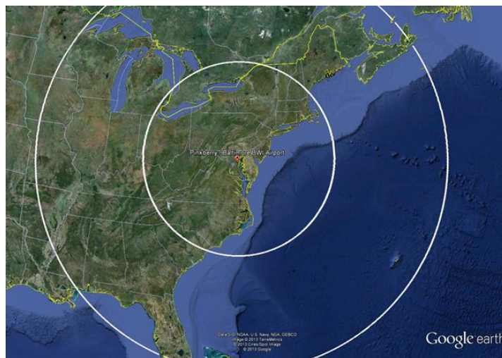
Figure 10. Map indicating the range of the C-130 aircraft for intensive research flights (inner circle) and those combining high altitude transit with low altitude cruising (outer circle).
