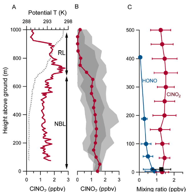
Figure 5. ClNO 2 and HONO mixing ratios as a function of height above ground surface in the Los Angeles basin during the CalNex 2010 campaign. A. Example vertical profile of ClNO 2 and potential temperature from the NOAA P-3 aircraft. B. Median (circles), 25 th and 75 th percentiles (dark shade) and 10 th and 90 th percentiles (light shade) from 21 nighttime profiles across the L.A. basin. C. Comparison of average ClNO 2 from P-3 profiles to average HONO from a multiple long-path DOAS instrument over the range 0-500 m. The DOAS was located in Pasadena, CA, while the ClNO 2 profiles were distributed throughout the L.A. Basin.
