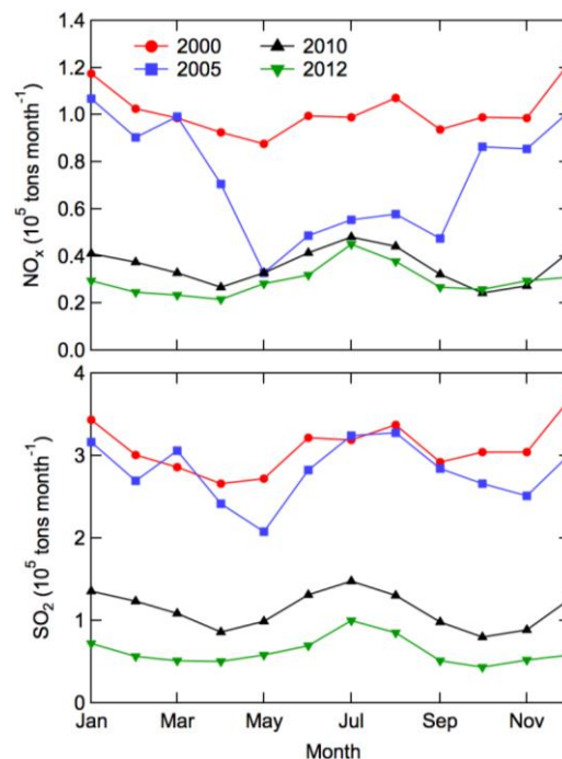
Figure 8. CEMS \text{NO}_x (Top) and \text{SO}_2 (Bottom) emissions from Northeast U.S. fixed location point sources (mainly power plants) for select years.
