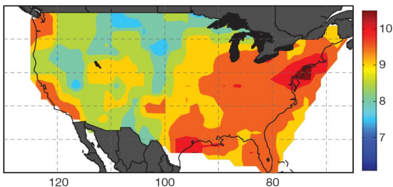
Figure 2. Predicted annual production rate of ClNO 2 is shown for the continental U.S. Color scale is logarithmic in units of gCl per 1°x1° grid cell per year. Adapted from Thornton et al. [2010]
