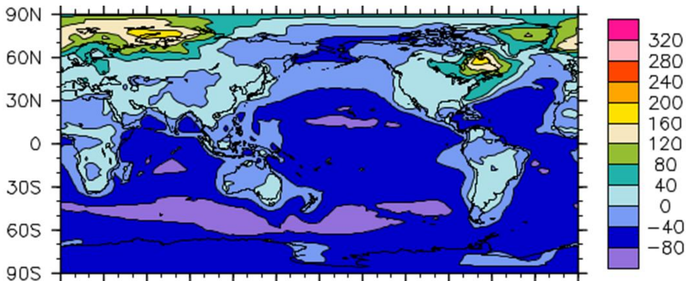
Figure 4. CAM simulations of the annual mean perturbation to \text{NO}_x abundance in the planetary boundary layer resulting from incorporation of full halogen chemistry [Long et al., 2013].
