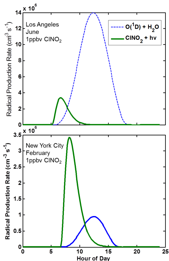
Figure 3. Example MCM box model calculations of the radical production rate from ClNO 2 and ozone photolysis for two cases of LA in June and NY City in February. For simplicity, the only differences between the two cases are the seasonal and latitude dependent photolysis frequencies, temperature, and water vapor mixing ratios. Otherwise, NO x , O 3 and VOC are assumed to be similar.
