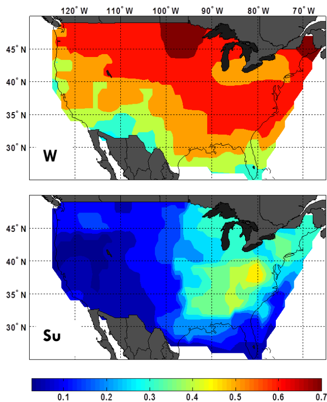
Figure 1. The fraction of total nitrate ( \text{HNO}_3 + \text{NO}_3^- ) formed over the U.S. from heterogeneous hydrolysis of \text{N}_2\text{O}_5 as predicted by the GEOS-Chem model for winter (W) and summer (Su).
