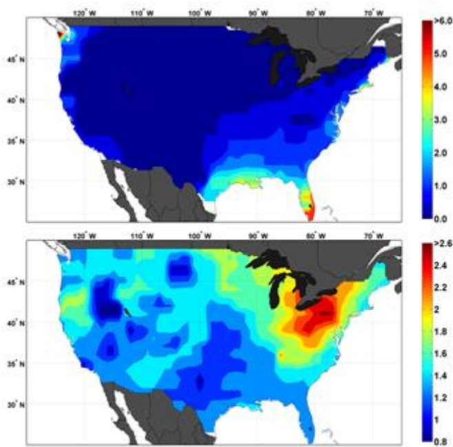
Figure 9. Annual mean (1996–2010) wet deposition of chloride (mg/yr, top) and the mole ratio of chloride to sodium (bottom) measured in precipitation by the National Atmospheric Deposition Program (NADP); ratios >1.2 are higher than that in seawater.
